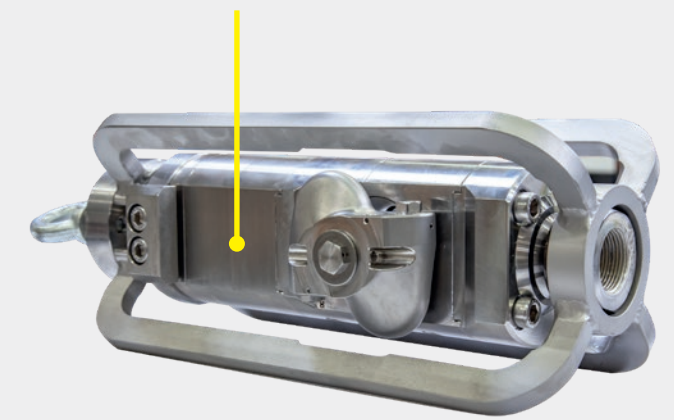
Central positioning of the AQUAMAT in the guide sledge
